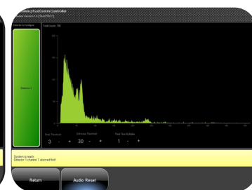
Barium-133 Spectra
