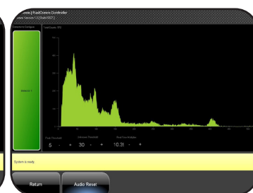
Thorium-232 Spectra
